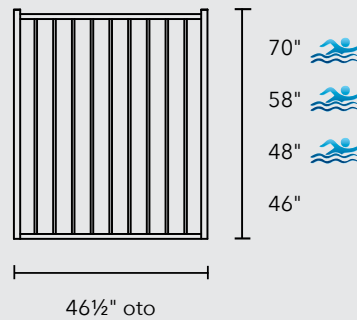
WALK GATE
