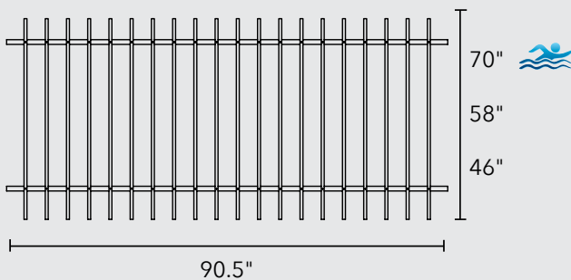
PANEL
