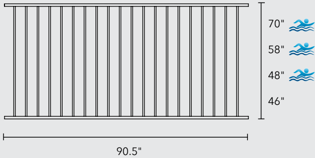
PANEL
