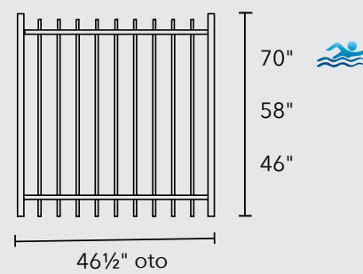
WALK GATE
